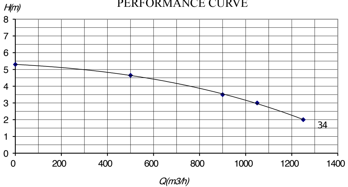
PERFORMANCE CURVE
