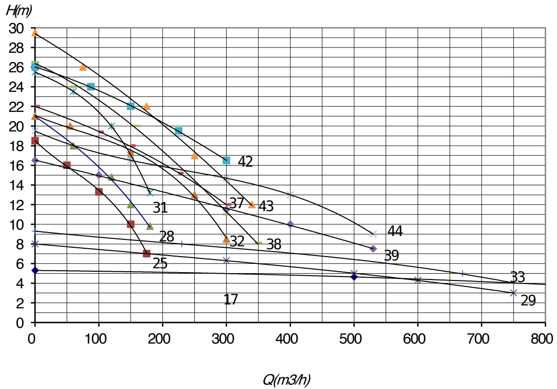
PERFORMANCE CURVE
